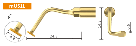
mUS1L Angled Micro-Saw 0.6mm. All the osteotomy techniques in maxilla and mandible; bone block grafting, horizontal osteotomy - left angle.
