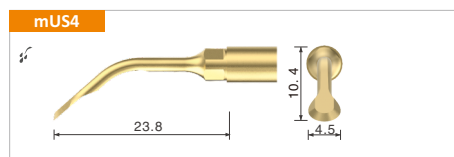
mUS4 Osteoplasty Scalpel. Universal osteoplasty, periodontal osteotomy, crown lengthening, bone chip harvesting, inflammatory tissue removal (cysts, etc.).
