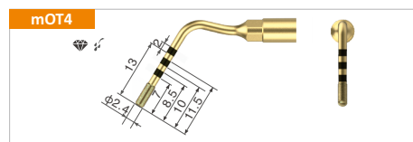
mOT4 Implant Site Preparation. To correct pilot osteotomy axis, to finalise the implant site preparation close to the alveolar nerve; sinus crestal approach techniques.
