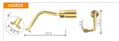
mUS1R Angled Micro-Saw 0.6mm. All the osteotomy techniques in maxilla and mandible; bone block grafting, horizontal osteotomy - right angle.
