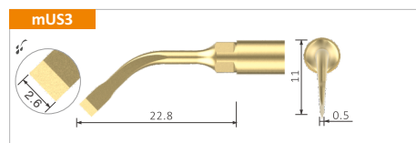
mUS3 Basic Scalpel. Osteotome of great precision in anatomically thin structures (for example ridge expansion, interdental corticotomies, nontraumatic nasal spina).
