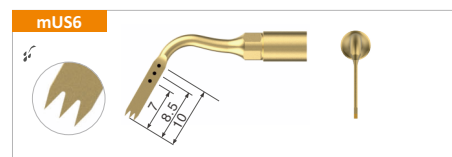
mUS6 Special Micro-Saw (3 teeth). Very thin and small osteotomy and corticotomy technique for orthodontic microsurgery, root fraction technique for dental extraction maneuver.
